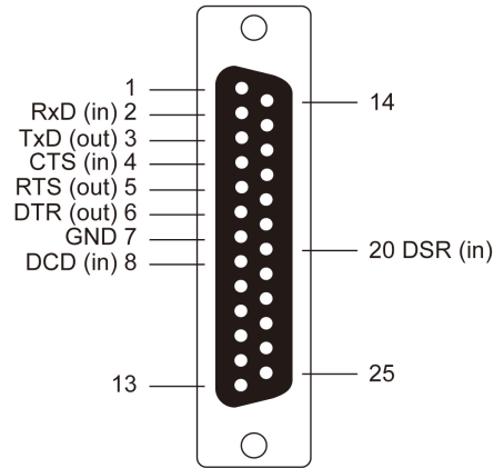
DB25 Female Connector
