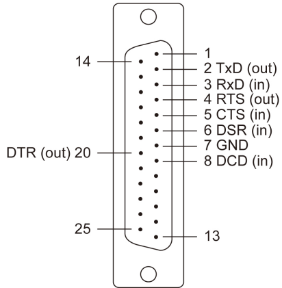
DB25 Male Connector
